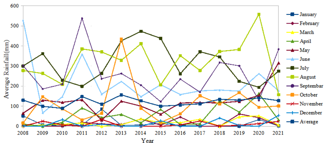
Fig. 18. Monthly average annual rainfall pattern in South Singhbhum region
