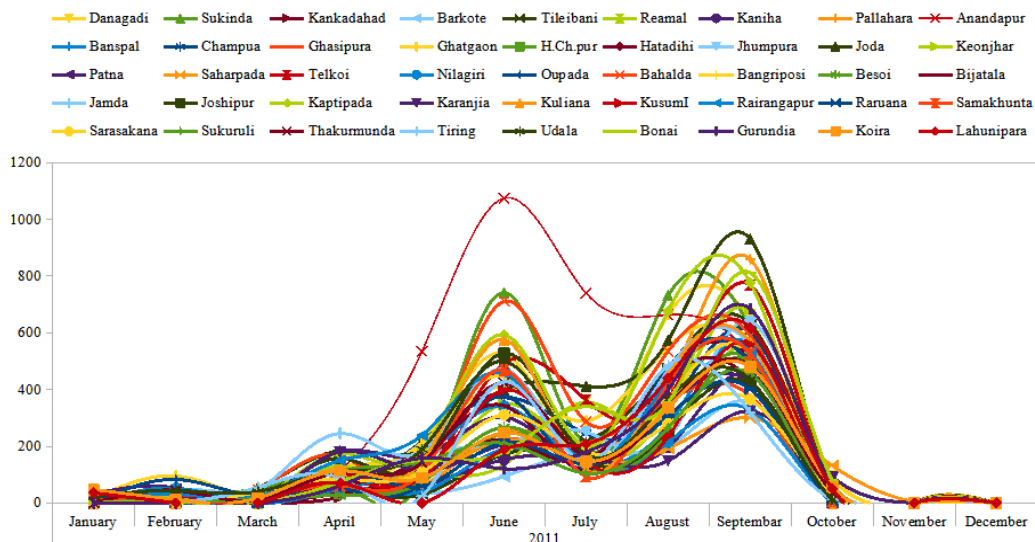
Fig. 7. Block wise monthly average rainfall of South Singhbhum Region in 2011
