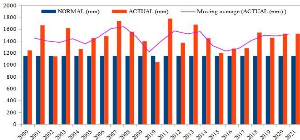
Fig. 2. Comparison between the normal and actual rainfall in Baitarani and Brahmani River Basin
