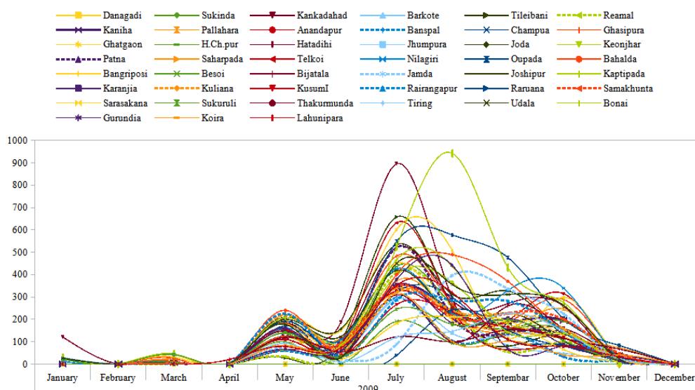
Fig. 5. Block wise monthly average rainfall of South Singhbhum Region in 2009
