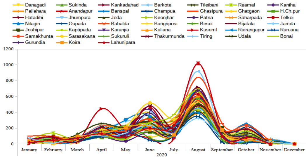
Fig. 16. Block wise monthly average rainfall of South Singhbhum Region in 2020
