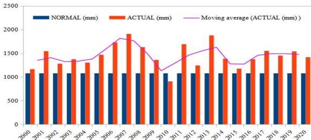
Fig. 3. Comparison between the normal and actual rainfall in Subarnarekha River Basin
