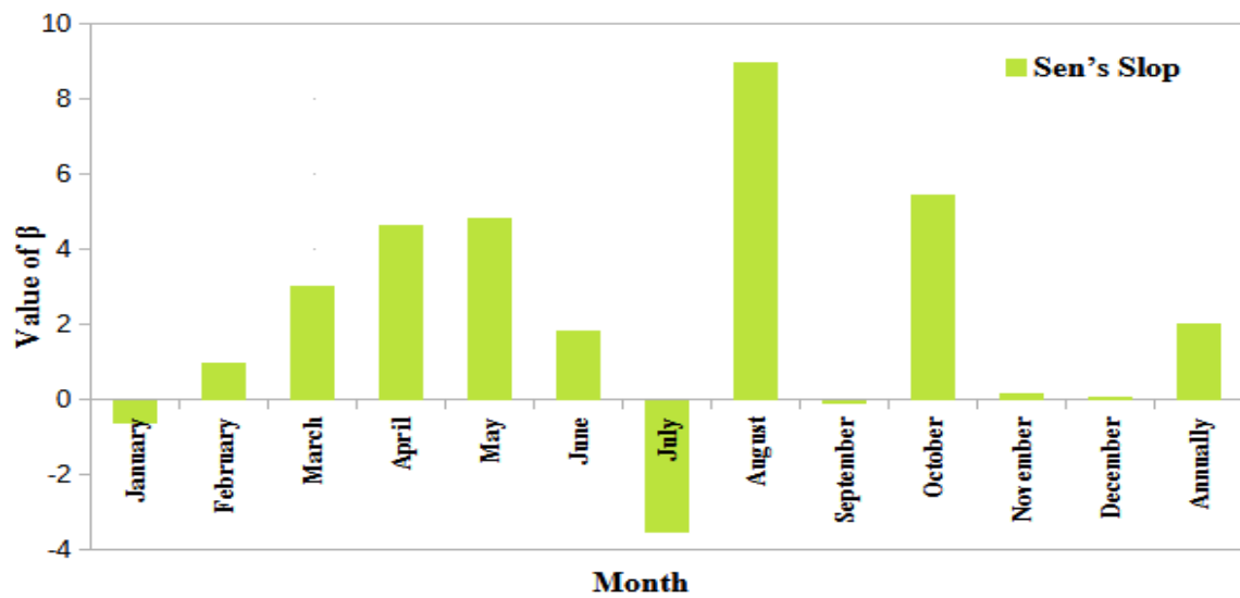
Fig. 19. Sen's Slop estimator for the monthly and annual rainfall in the south Singhbhum region
