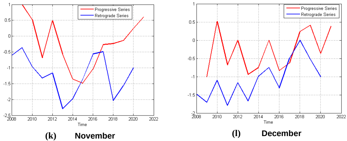
Fig. 20(a-l). Sequential Mann-Kendall test for monthly average rainfall in south Singhbhum region
