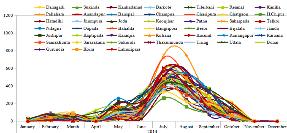
Fig. 10. Block wise monthly average rainfall of South Singhbhum Region in 2014
