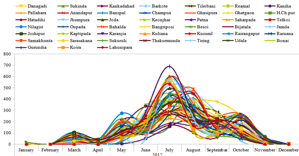
Fig. 13. Block wise monthly average rainfall of South Singhbhum Region in 2017
