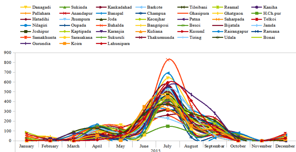
Fig. 11. Block wise monthly average rainfall of South Singhbhum Region in 2015
