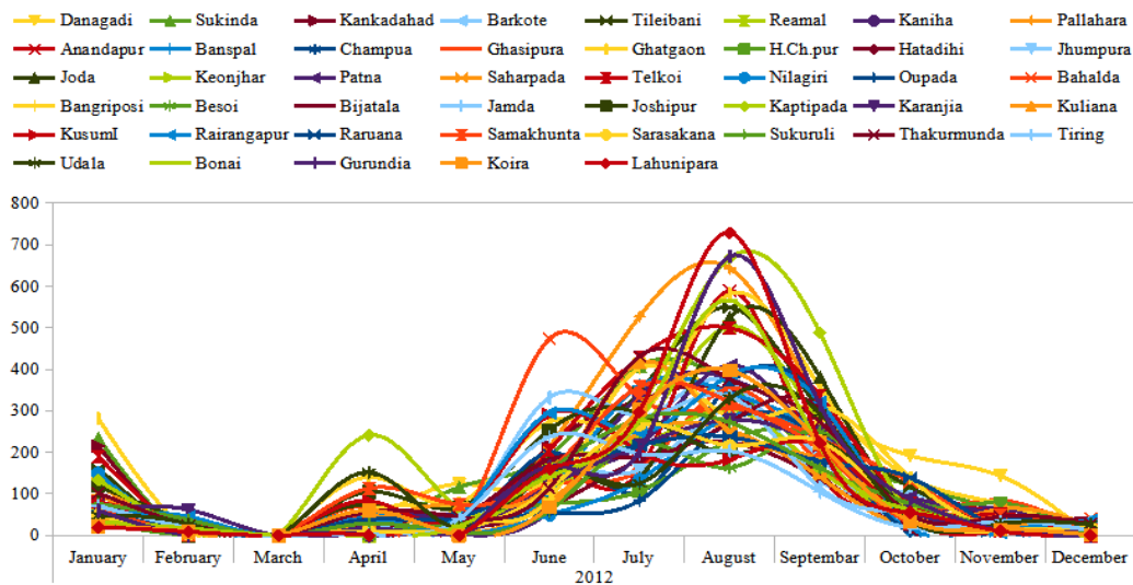
Fig. 8. Block wise monthly average rainfall of South Singhbhum Region in 2012
