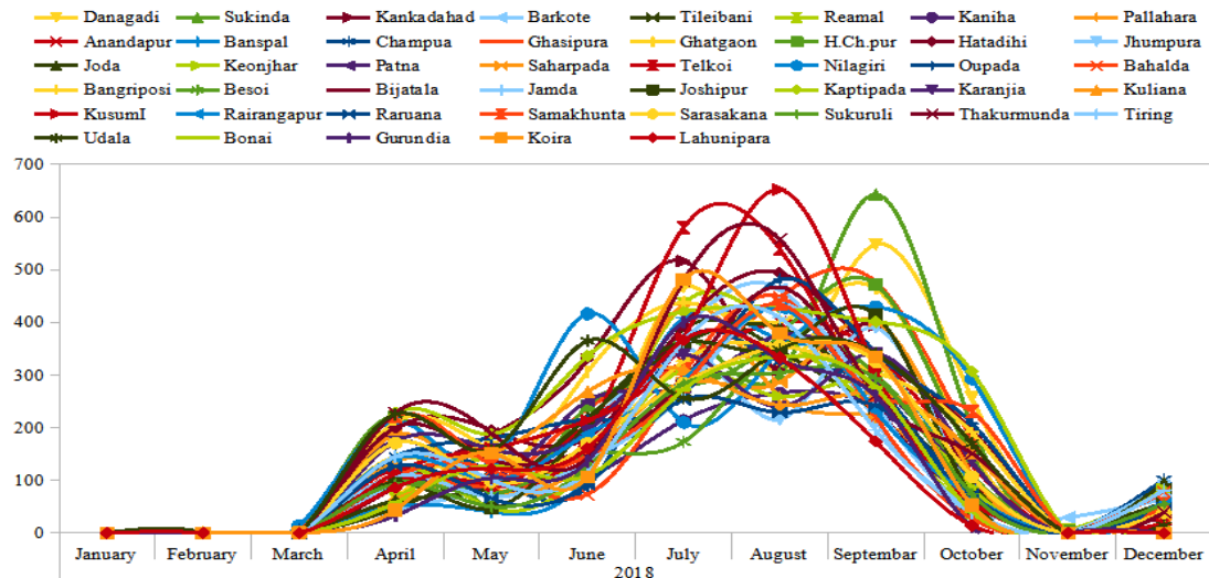
Fig. 14. Block wise monthly average rainfall of South Singhbhum Region in 2018
