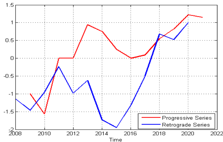
Fig. 21. Sequential Mann Kendall Test for annual average rainfall in the south Singhbhum region
