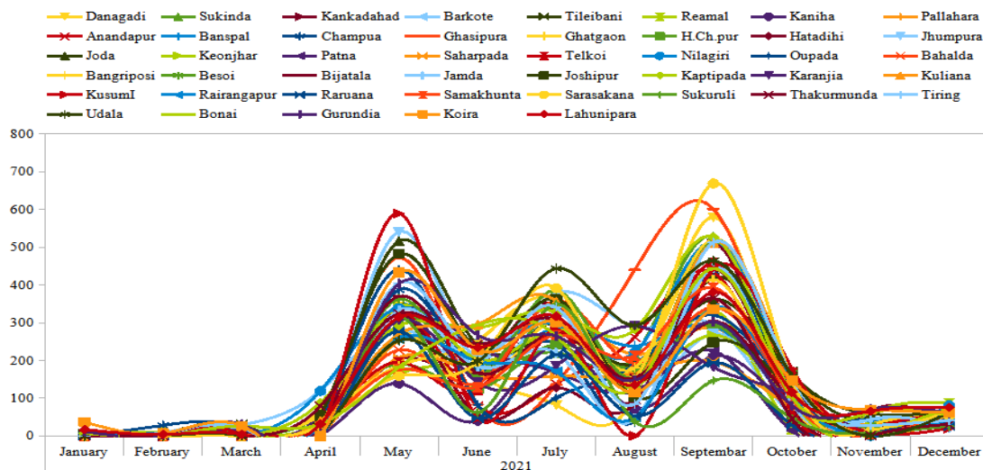
Fig. 17. Block wise monthly average rainfall of South Singhbhum Region in 2021
