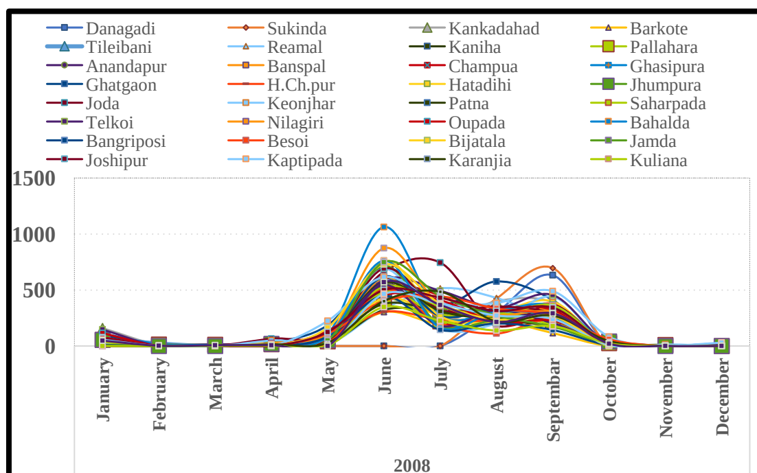
Fig. 4. Block wise monthly average rainfall of South Singhbhum Region in 2008
