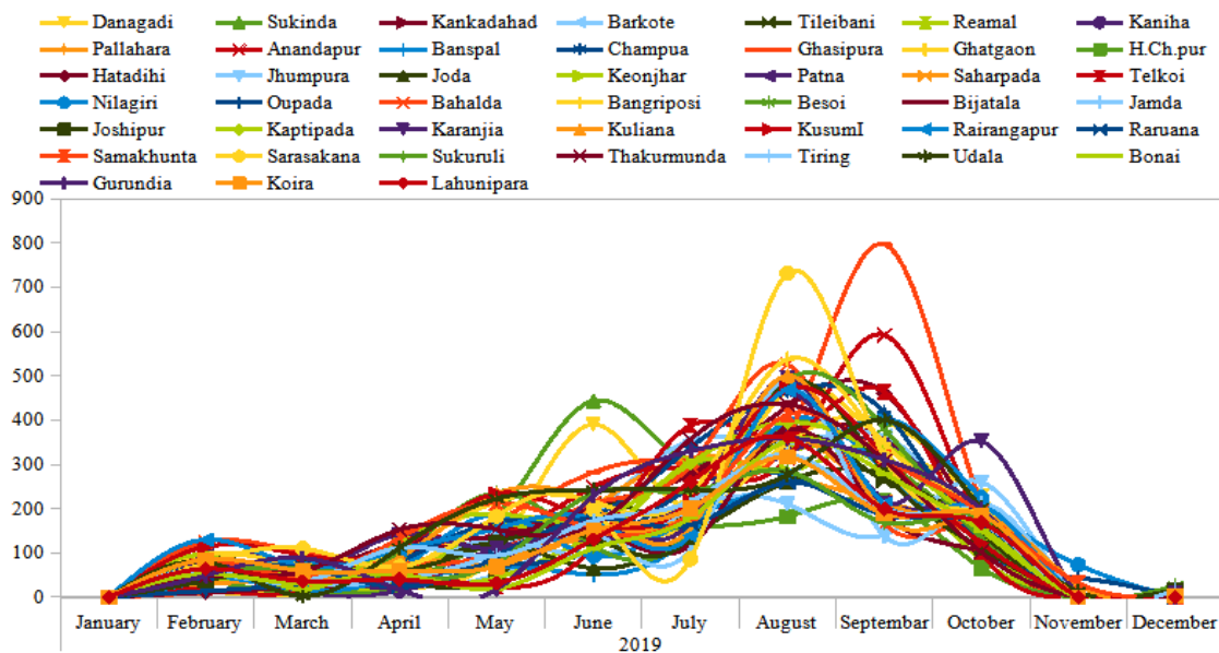
Fig. 15. Block wise monthly average rainfall of South Singhbhum Region in 2019
